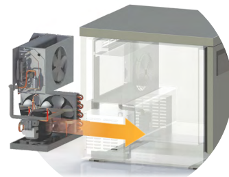
Back Mount
